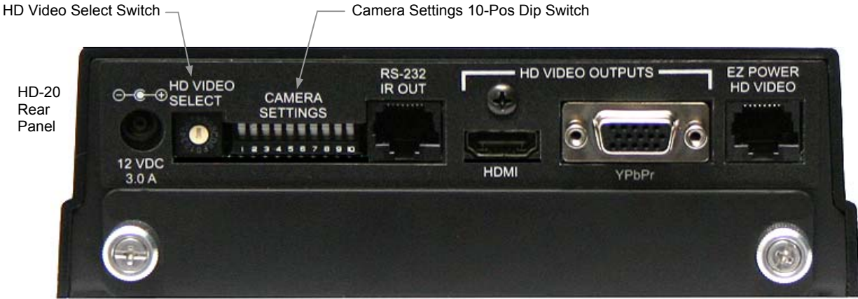
Label on Bottom of HD-20
